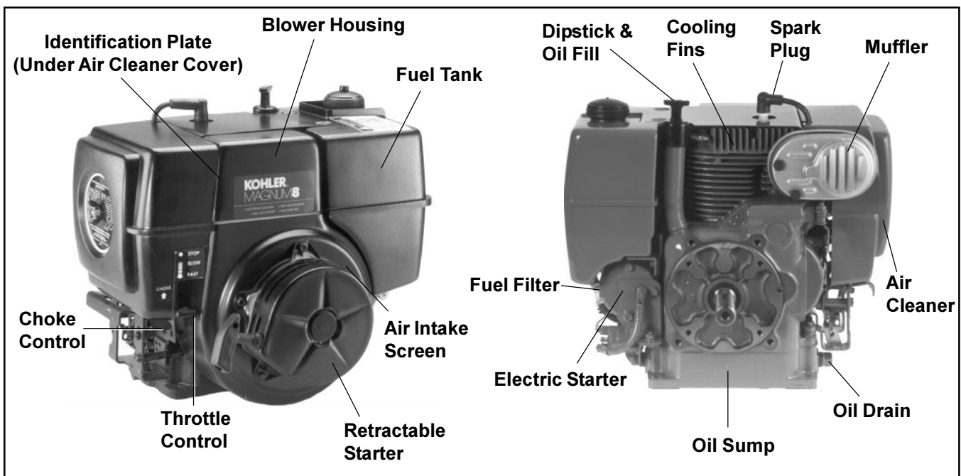
Figure 1. Typical Model M8 Engine.
